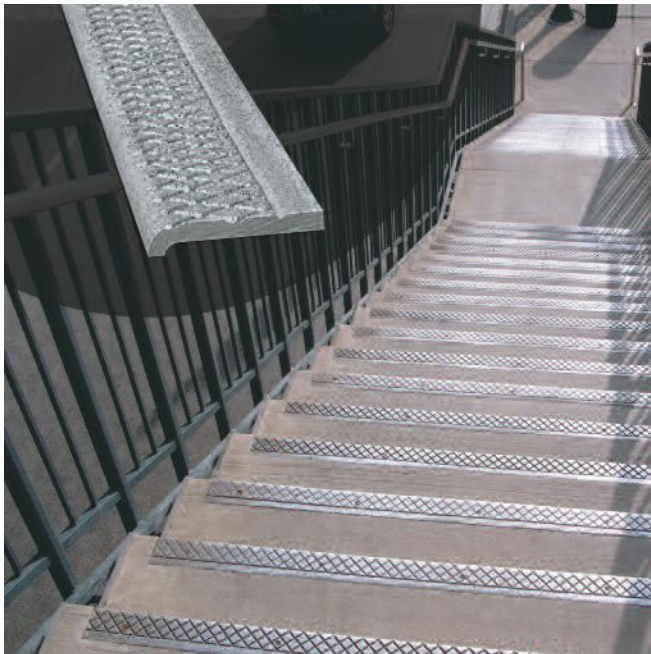
TYPE 116A – Nose depth 1" (25.4 mm) standard. Chief use: on top of existing steps for repair and modernization.
