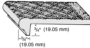
TYPE 103 – Nose 3/4" x 3/4" (19.05 mm x 19.05 mm). Chief use: as structural treads with bent-plate risers or as nosings full width of stair.
