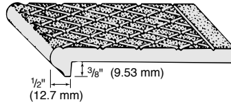
TYPE 102 – Nose 1/2" x 3/8" (12.7 mm x 9.53 mm). Chief use: as nosings on steel-pan stairs. Can also be used structurally with bent-plate risers.
