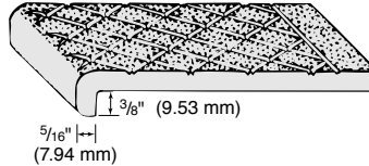
TYPE 101SP – Nose 3/8" (9.53 mm). Chief use: as nosings on steel-pan concrete-filled stairs or on existing steps.
