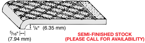
TYPE 101 – Nose 5/16" (6.35 mm) lip. Chief use: as nosings, formed concrete stairs. Tread installed flush all around.
