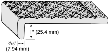
TYPE 116A – Nose depth 1" (25.4 mm) standard. Chief use: on top of existing steps for repair and modernization.
