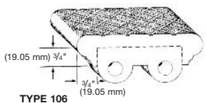
TYPE 106 Double nose tread, reversible. End lugs provided for bolting treads directly to stringers.
