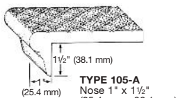
TYPE 105-A Nose 1" x 1 1/2" (25.4 mm x 38.1 mm)
