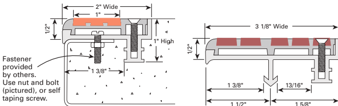
TYPE WP-RN2SG 2" (50.8 mm) wide, 1/2" (12.7 mm) thick
