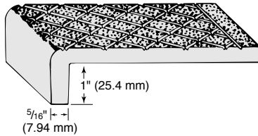
TYPE 116 – Nose depth 1" (25.4 mm) standard. Chief use: as nosings, formed concrete stairs where deeper lip is desirable.
